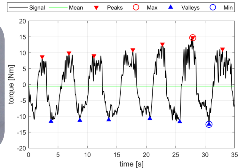
Measurement of the torsional load acting on the shell during skiing with a skier
