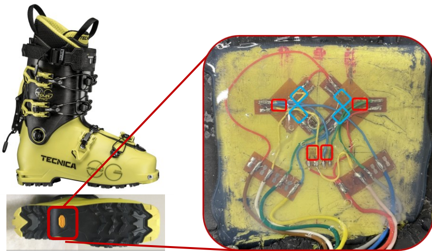
Preparation of the boot with strain gauges
